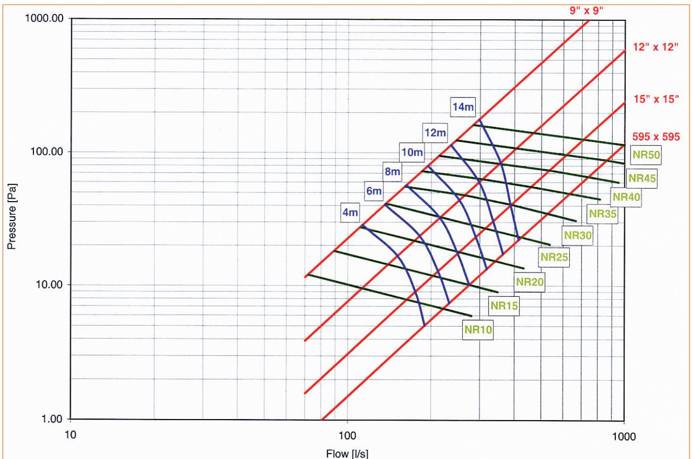
CD2000 - Plastic Square Ceiling Diffuser Selection Nomogram Pressure Drop vs Flow vs Throw vs NR
