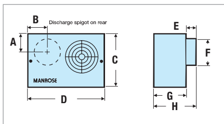
▶ Dimensions - CF200
