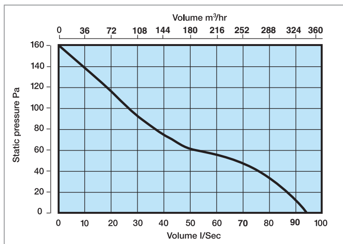
▶ Performance - ELLP150
