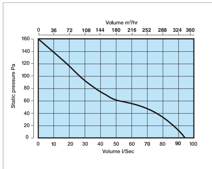
▶ Performance - SFLP150
