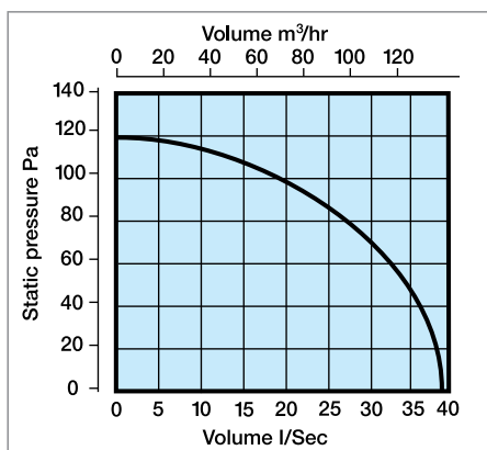
▶ Performance - CFD200
