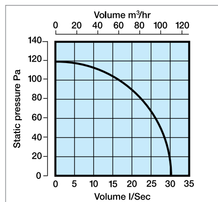
▶ Performance - CFD225
