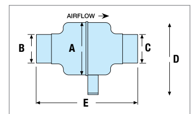
▶ Dimensions - CFD200/CFD225
