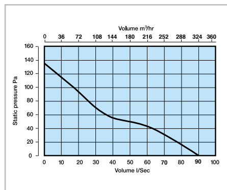
▶ Performance - 150mm Frame Fan
