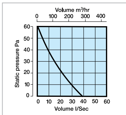
▶ Performance - 125mm Frame Fan
