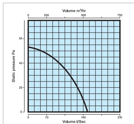
▶ Performance - XFS230
