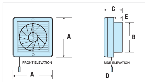
▶ Dimensions - XF230/300
