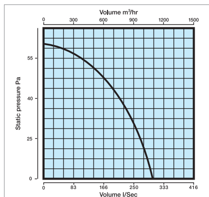
▶ Performance - XFS300
