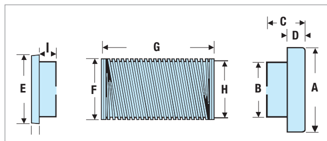
▶ Dimensions - XPS230/300
